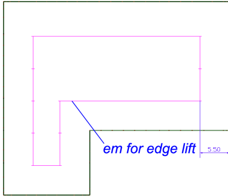
(a) Plan Showing E_m For Edge Lift Condition
