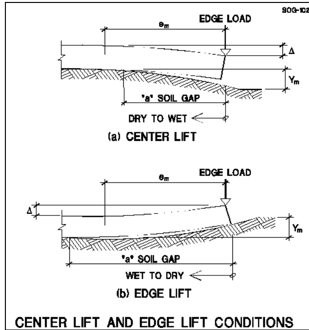
CENTER LIFT AND EDGE LIFT CONDITIONS
