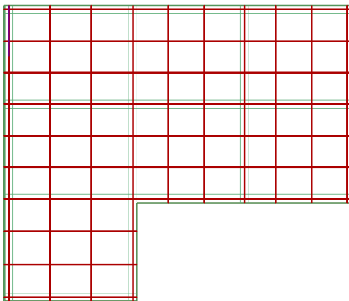
(a) Layout of Tendons in Plan
