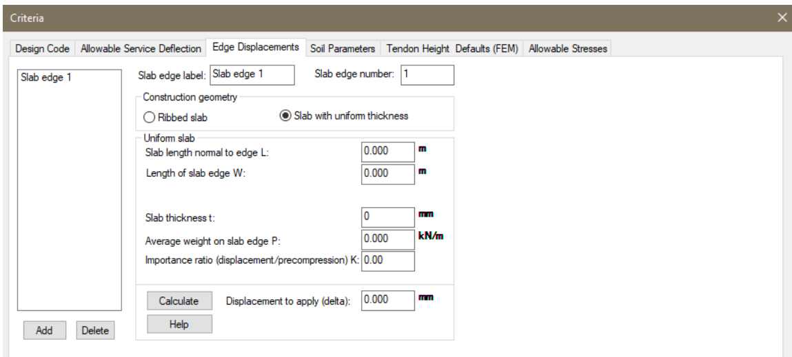
Figure 3.3-3 - Input Dialog Window for the Calculation of Applied Edge Displacement \Delta for Slabs with Uniform Thickness
