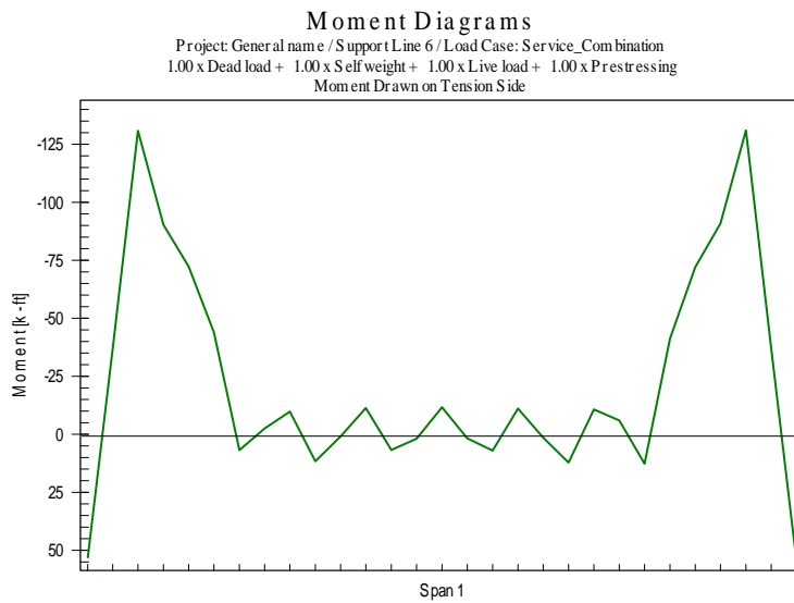
Figure 5.6-5 - Distribution of Moment for Design Strip 6 (The positive moment at either end is due to the Tendon eccentricity at the edge Beam; the steps in the moment diagram are due to transfer of torsion at interior cross Beams.)
