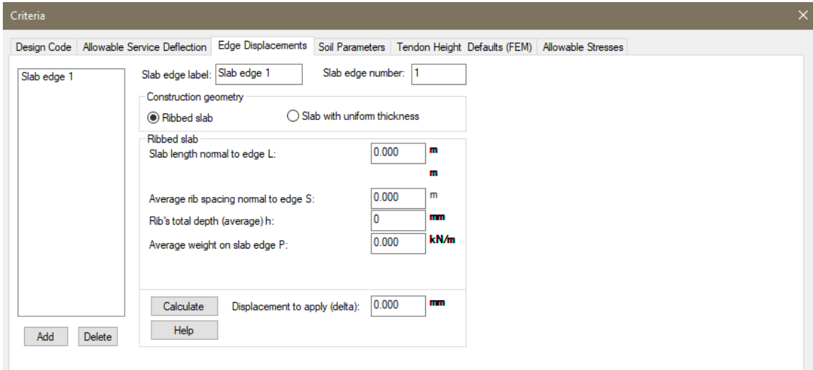
Figure 3.3-4 - Input Dialog Window for The Calculation of Applied Edge Displacement \Delta for Ribbed Slabs
