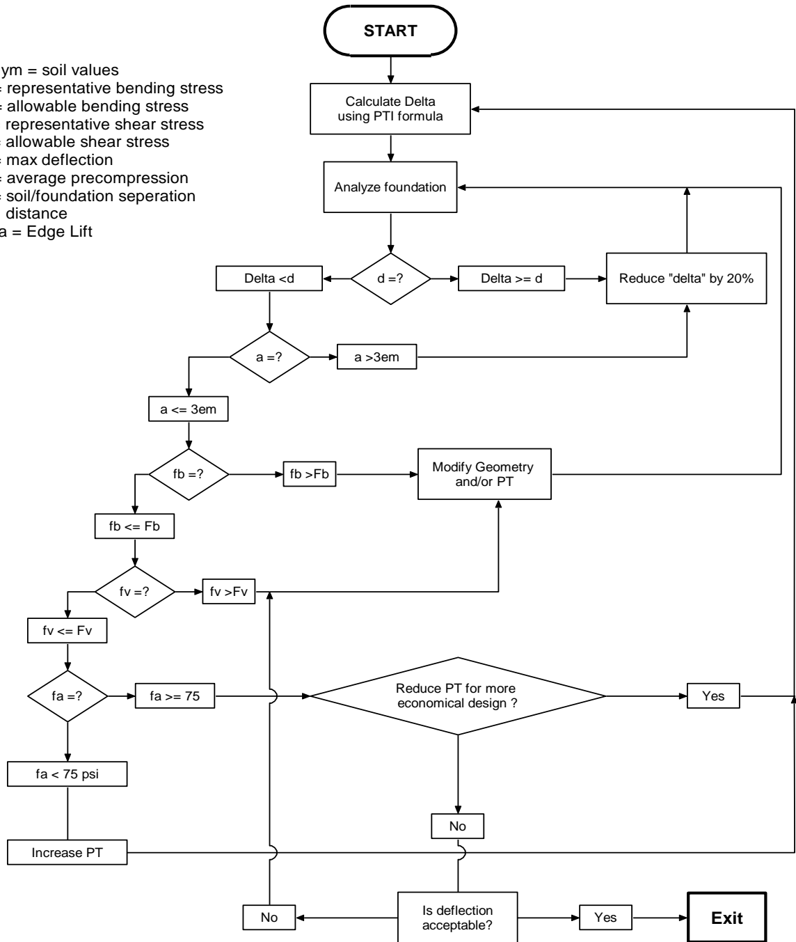
Figure 4.3.1-3 Flow Chart Of Edge Lift Design Procedure
