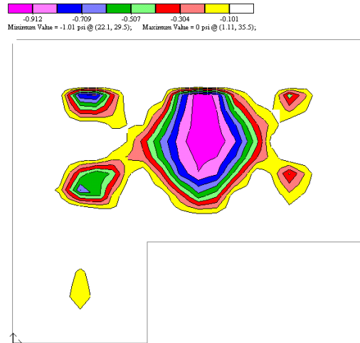
Figure 5.5-16 - Distribution of Soil Pressure for Edge Lift Equal to 0.05"
